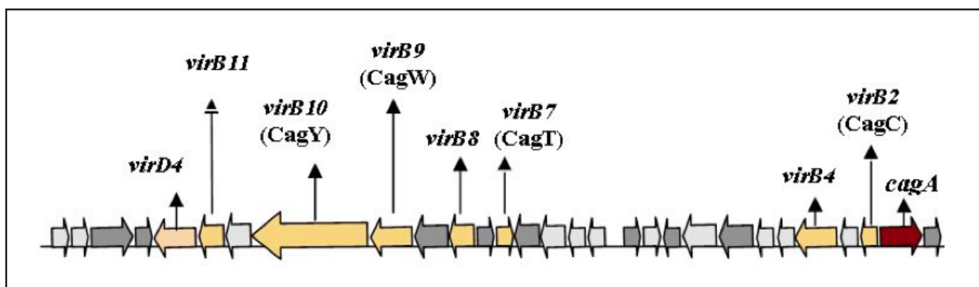
FIGURE 3. Genetic organization of cag pathogenicity island (PAI).
