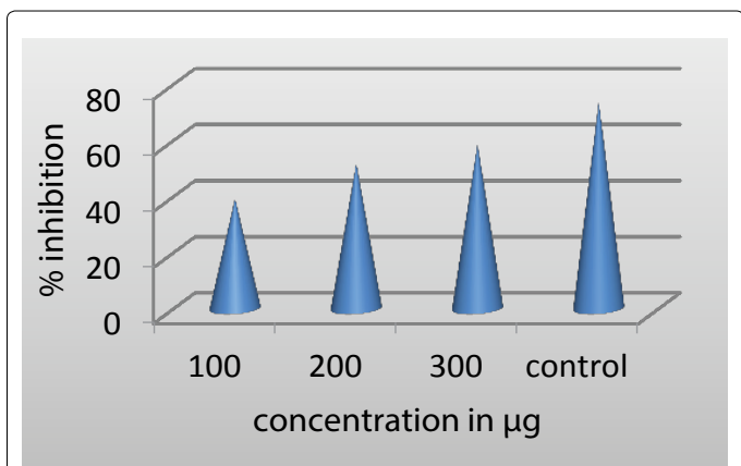
Figure 4: Effect of ethanolic extract of roots of Pergularia daemia on heat induced hemolysis for anti-inflammatory activity.
