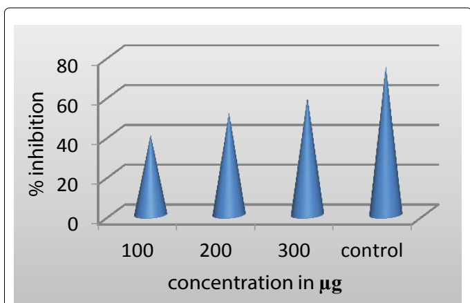
Figure 5: Effect of ethanolic extract of roots of Pergularia daemia on protein denaturation assay for antiarthritic activity.
