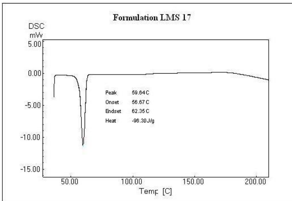
Figure 6: DSC of Best Formulation LMS 17
