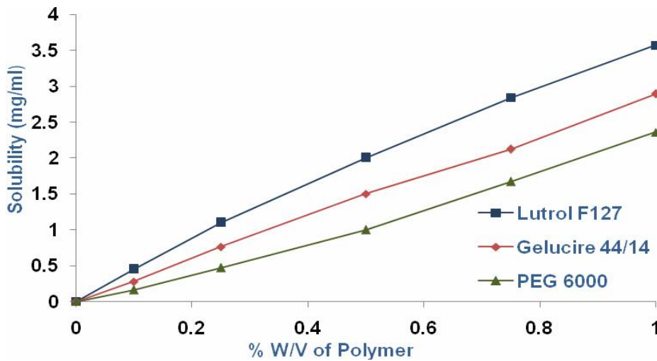
Figure 1: Phase Solubility Diagrams of Repaglinide
