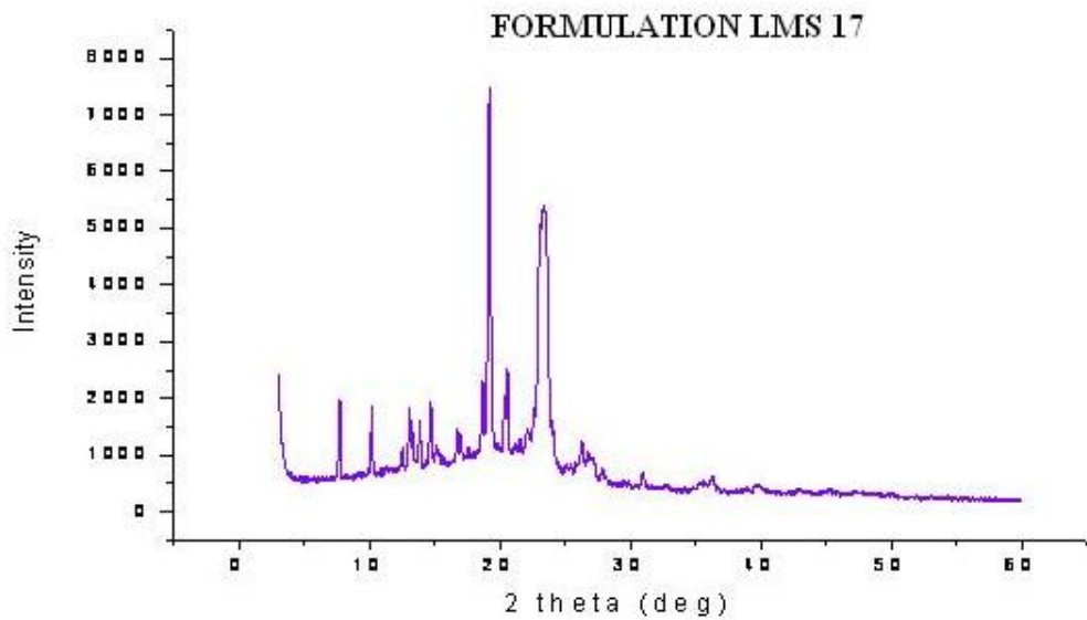
Figure 4: XRD of Best Formulation LMS 17
