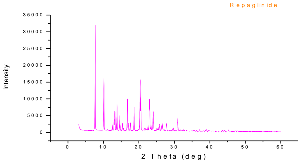
Figure 3: XRD of Repaglinide
