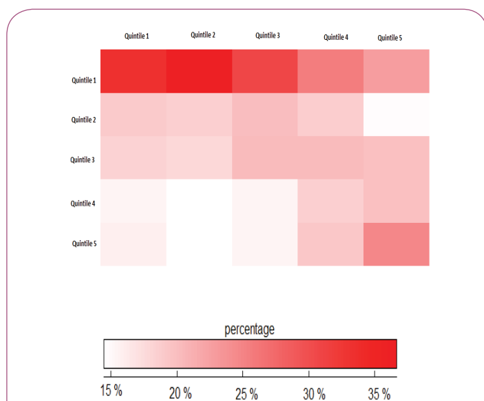
Figure 1 Results of hepatitis B surface antigen testing on the Abbott PRISM assay for donor (rows) and quality control (columns) samples sorted into quintiles with column percentages
