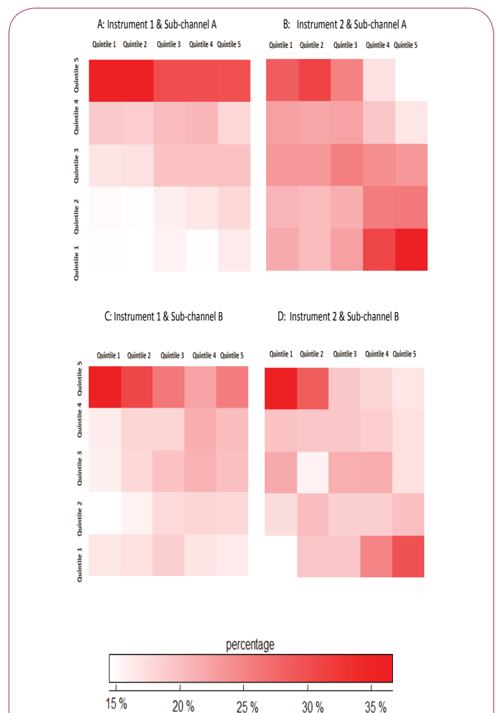
Figure 2 Results of hepatitis B surface antigen testing on the Abbott PRISM assay for donor (rows) and quality control (columns) samples sorted into quintiles with column percentages by Instrument (1 or 2) and sub channel (A or B)
